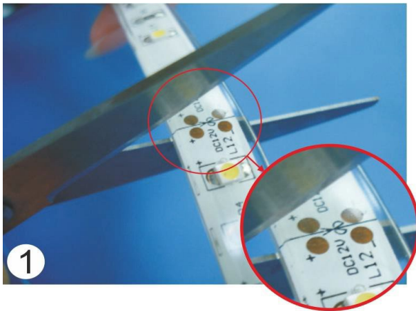
1 Cut the Flex Strip on marked cutting line.
