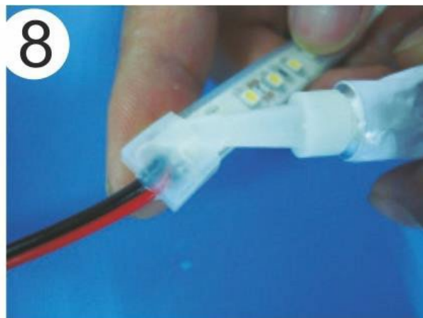
Fill the end cap completely with the glue.
