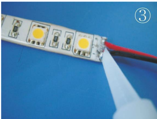
Cover the soldering point with acid free silicone for example PROLED sealing glue L6396.
