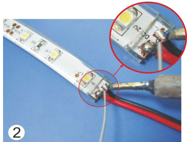
2 Remove the silicone from the soldering pads. Solder the cable correctly. Please take care about correct polarity.
