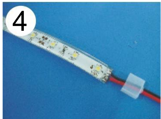
4 Move the end cap over the cable.
