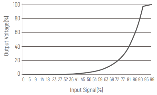
0/1-10V Curve
