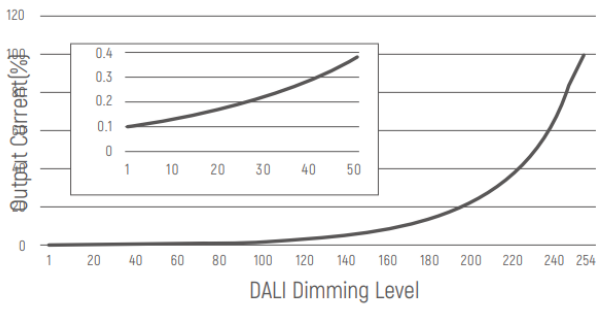
DAI Curve
